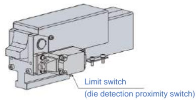
Automatic slidable type with limit switch (Die detection proximity switch)
