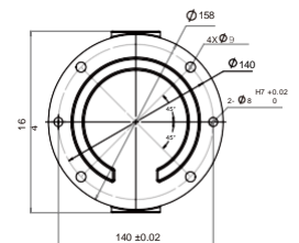
JAKA Zu ® 5 P point front view / top view
