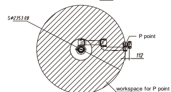
JAKA Zu ® 12 P point front view / top view
