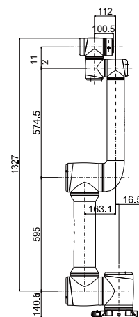
JAKA Zu ® 12 work radius
