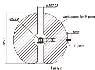
JAKA Zu ® 12 work radius
