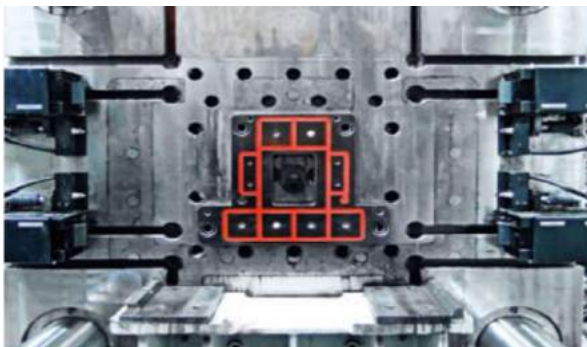
8,500kN (850ton) Die-casting machine C-plate mag clamp & Hydraulic clamp TYB-Z
